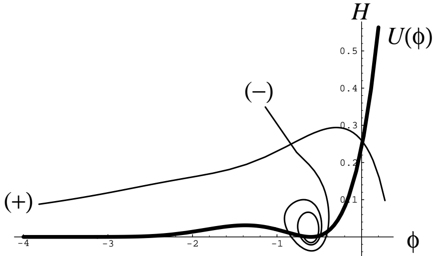
Figure 1. The potential U(\phi) and trajectories of (+) and (-) branches. The (-) branch settles down at a minimum of the potential.
